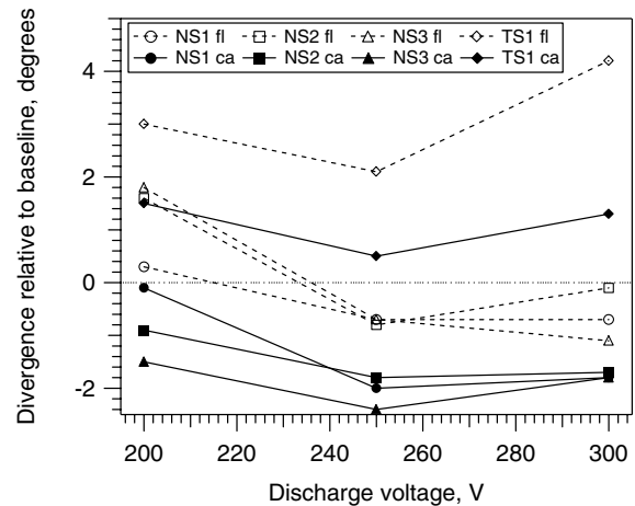
Fig. 7 Divergence ( \pm 1 deg) relative to baseline with BN coat on outer magnetic pole.
