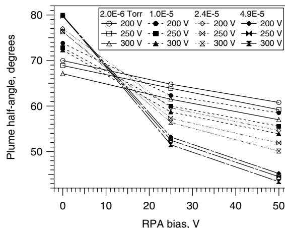
Fig. 10 Baseline divergence ( \pm 1 deg) as a function of chamber background pressure at 250 V.
