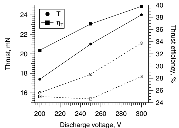
Fig. 3 Baseline thrust ( \pm 1 mN) and efficiency ( \pm 10\% ). Closed symbols: B set for minimum plume divergence; open symbols: B set for maximum divergence without unstable operation.
